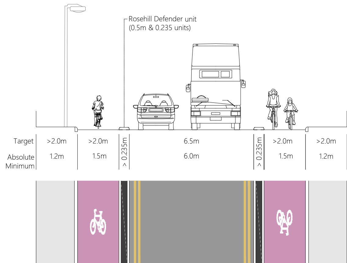
With-flow segregated cycle track
