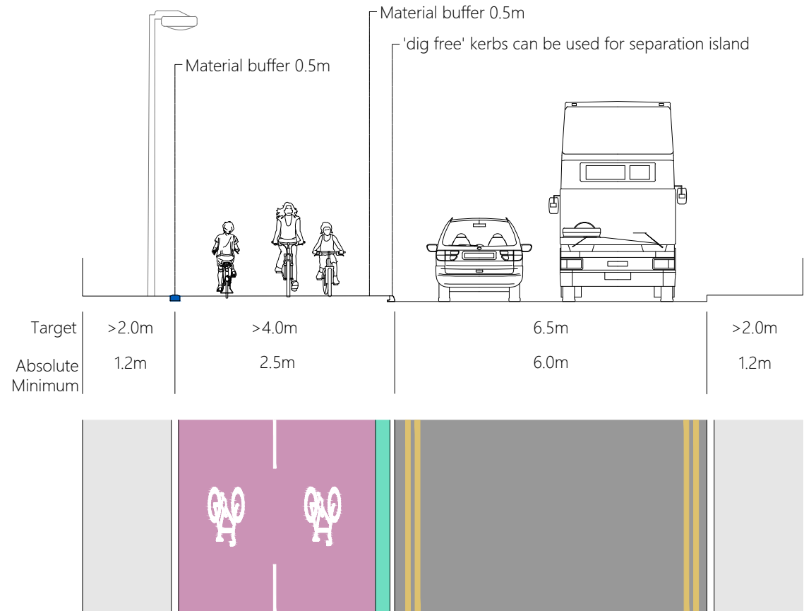
Two-way segregated cycle track
