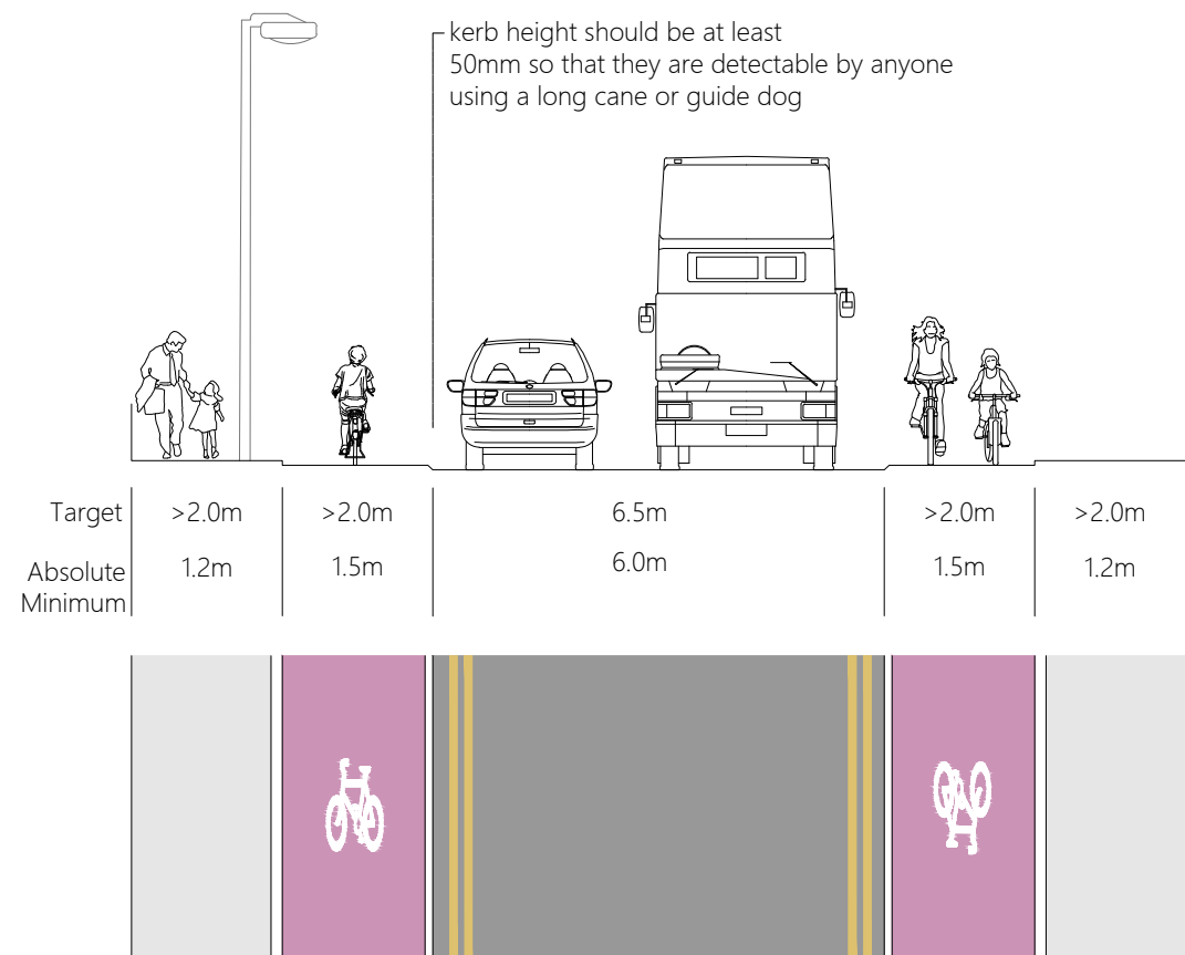
Stepped cycle track
