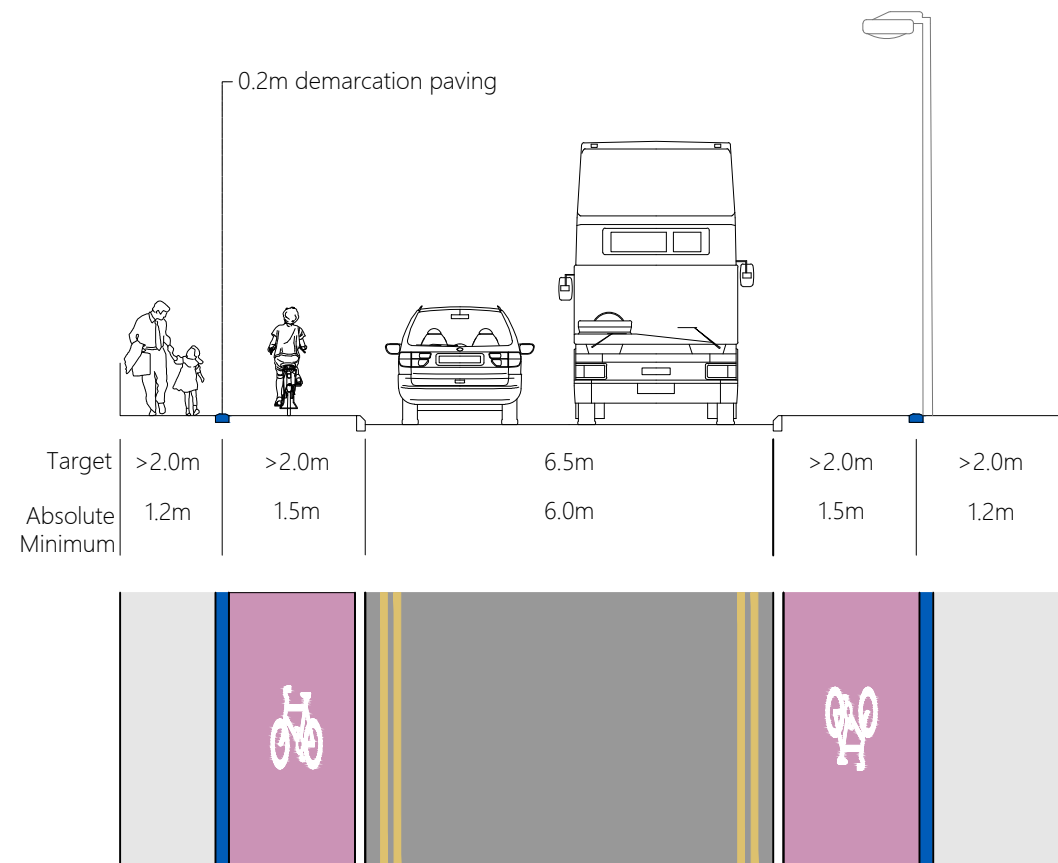
Footway level cycle track
